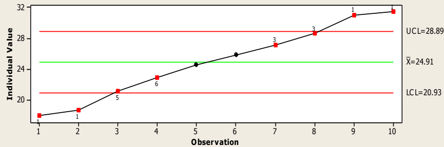
I-MR Chart of Foot
